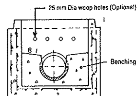
BENCHING DETAIL (Optional)
