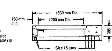
SECTION A-A TRANSITION SLAB
