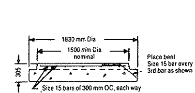
SECTION A-A BASE SLAB
